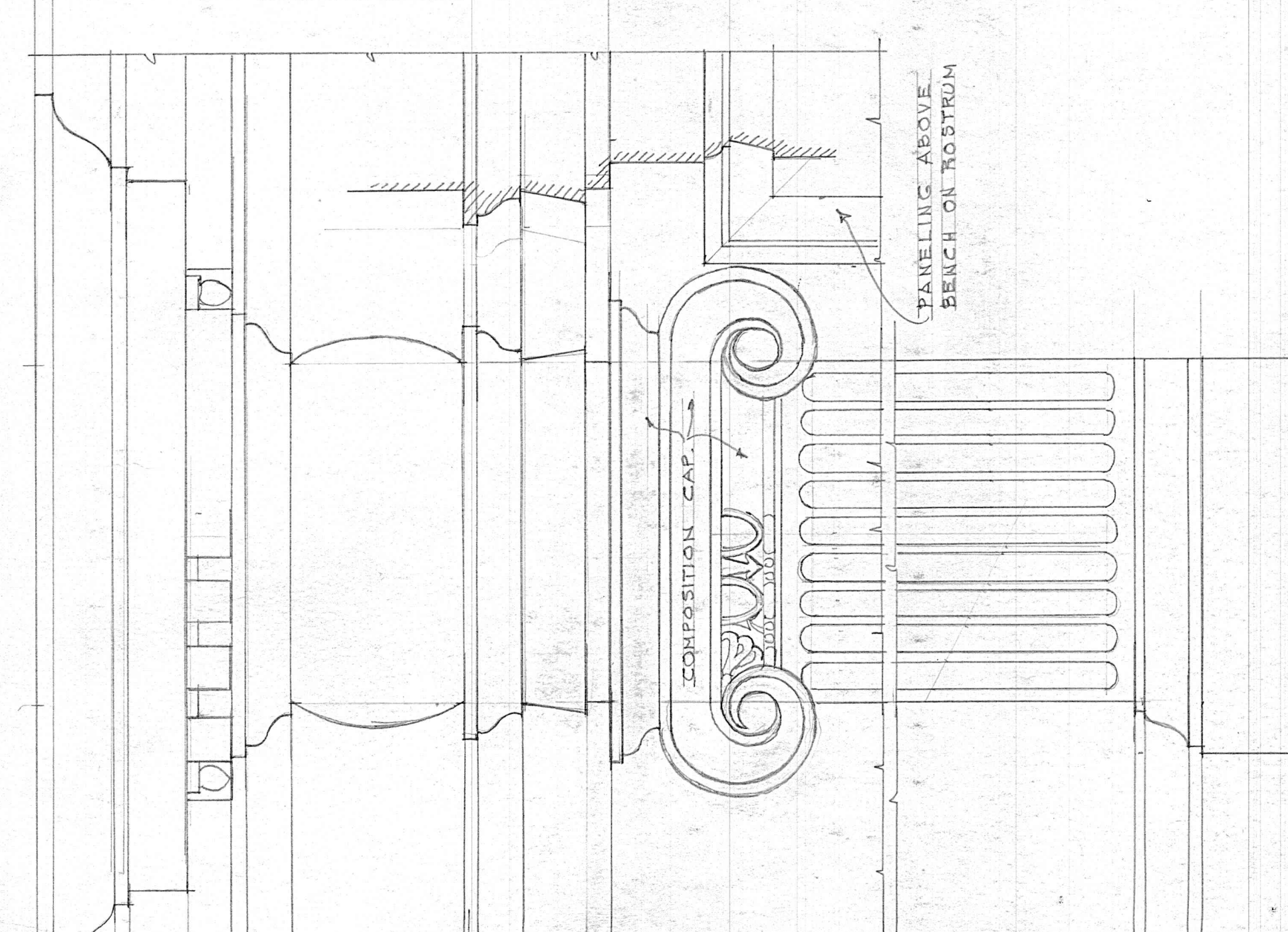
ELEV. DETAIL, PILASTER AND CORNICE IN ROSTRUM
