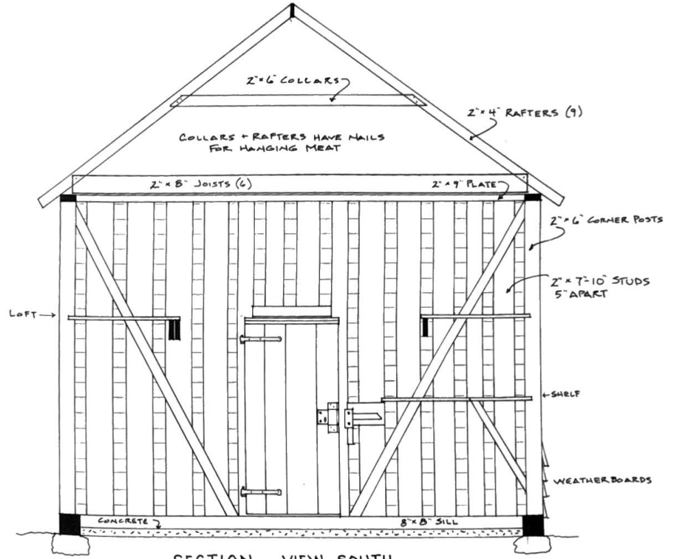
SECTION - VIEW SOUTH
