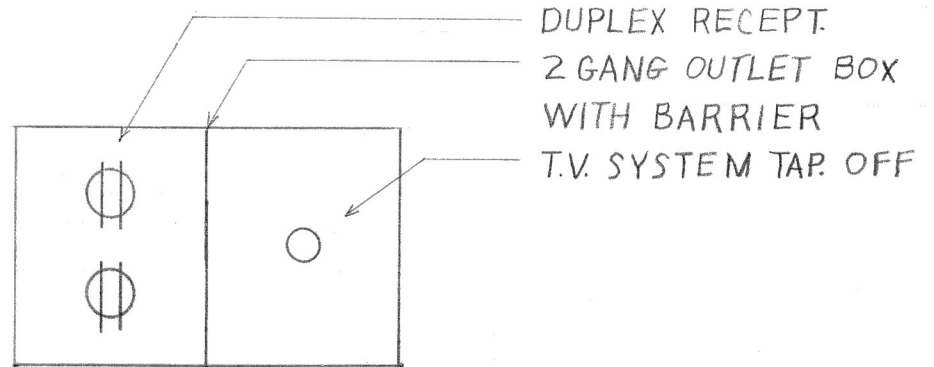
TYPICAL T.V. OUTLET
