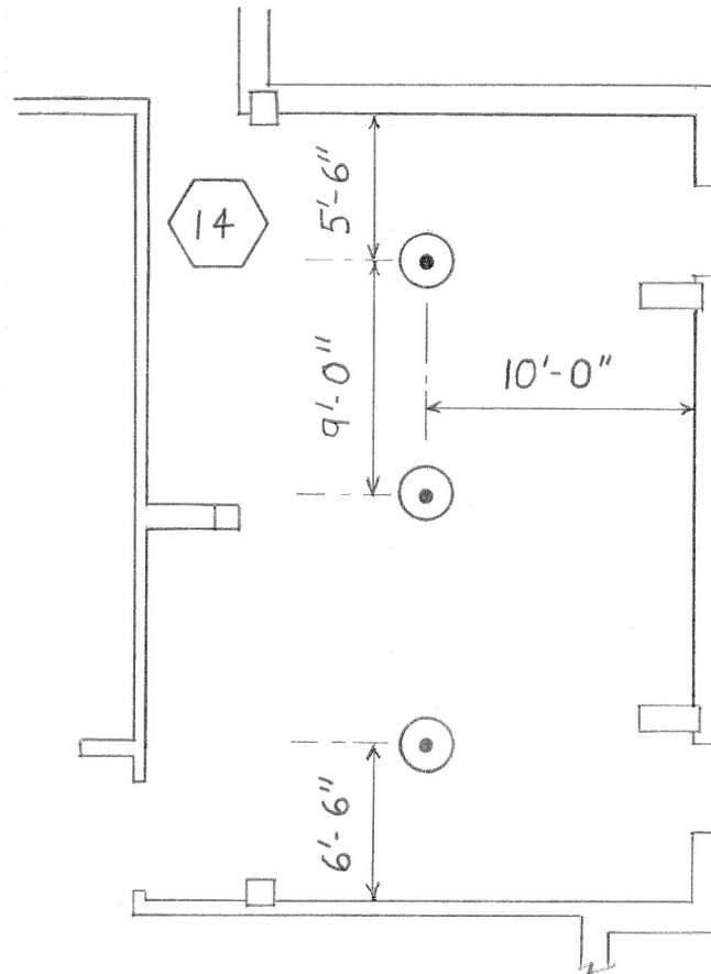
FLOOR OUTLET LOCATIONS
