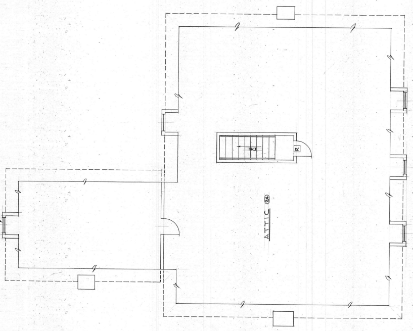
ATTIC FLOOR PLAN - CASKIE, SCRUGGS, SHELTON & PAXTON COTTAGES 1/4" = 1'-0"
