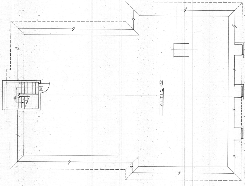
ATTIC FLOOR PLAN - NOBLE COTTAGE 1/4" = 1'-0"
