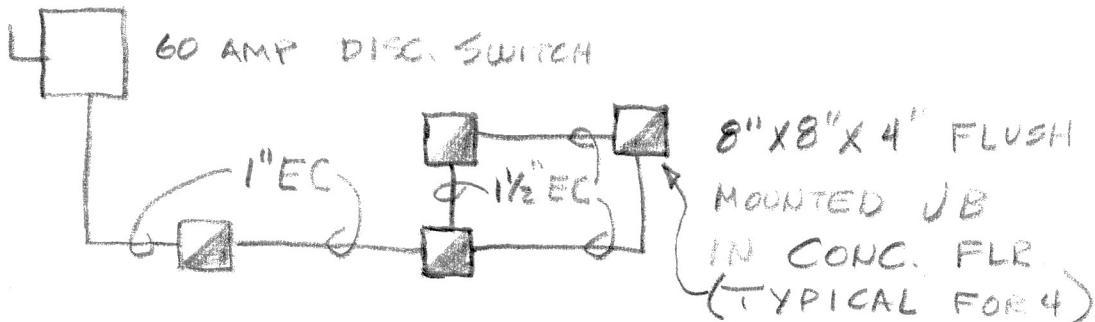
RISER DIAGRAM
