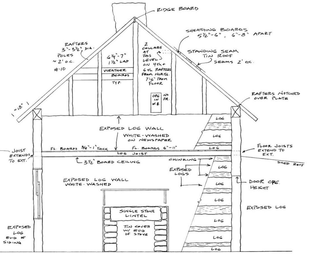
E-W SECTION VIEW NORTH
