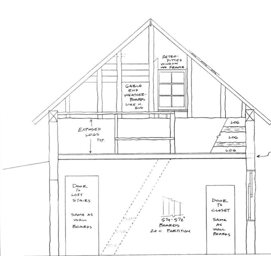
E-W SECTION VIEW SOUTH
