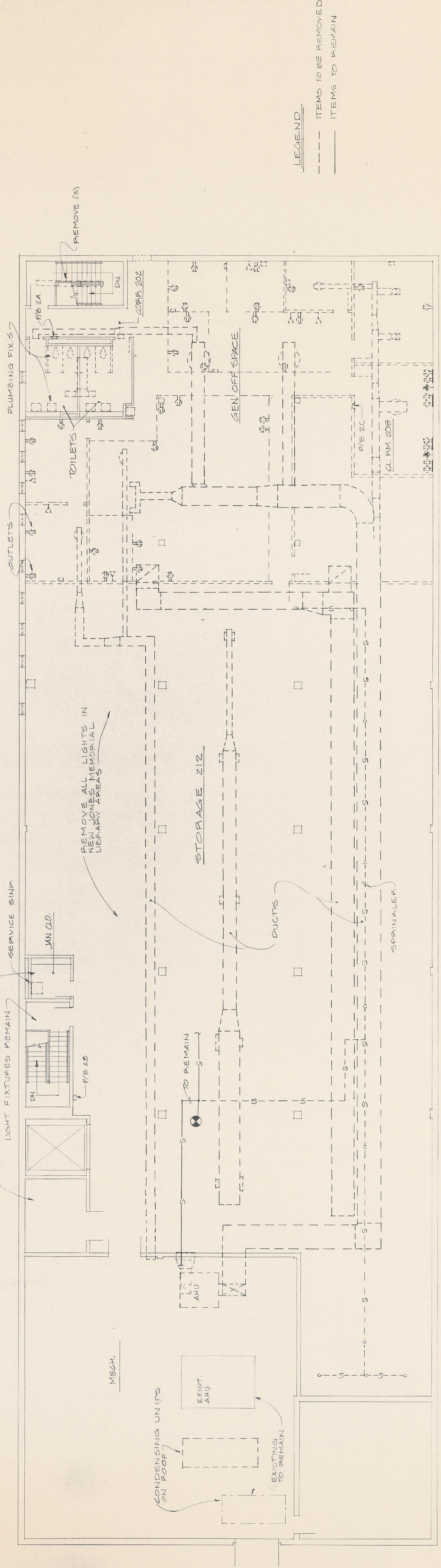
DEMOLITION - SECOND FLOOR PLAN SCALE: 1/8" = 1'-0"
