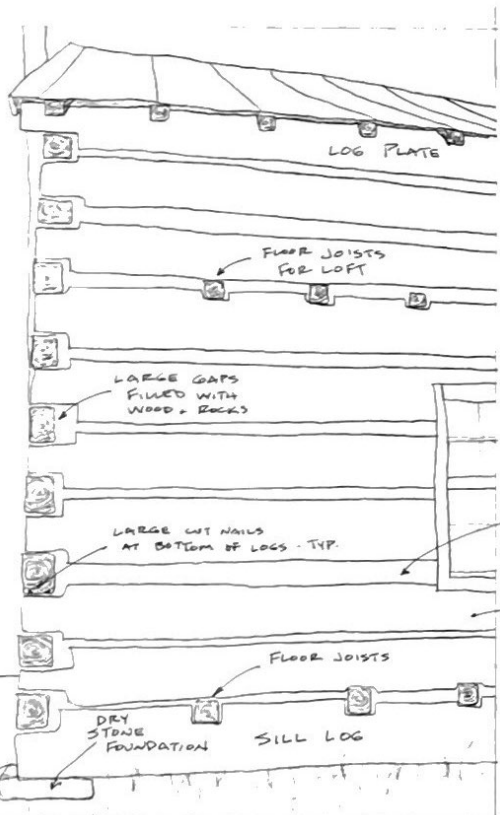
TYPICAL SQUARE NOTCH CONSTRUCTION OF CABIN (NORTHWEST CORNER, FROM PHOTO) N.S.
