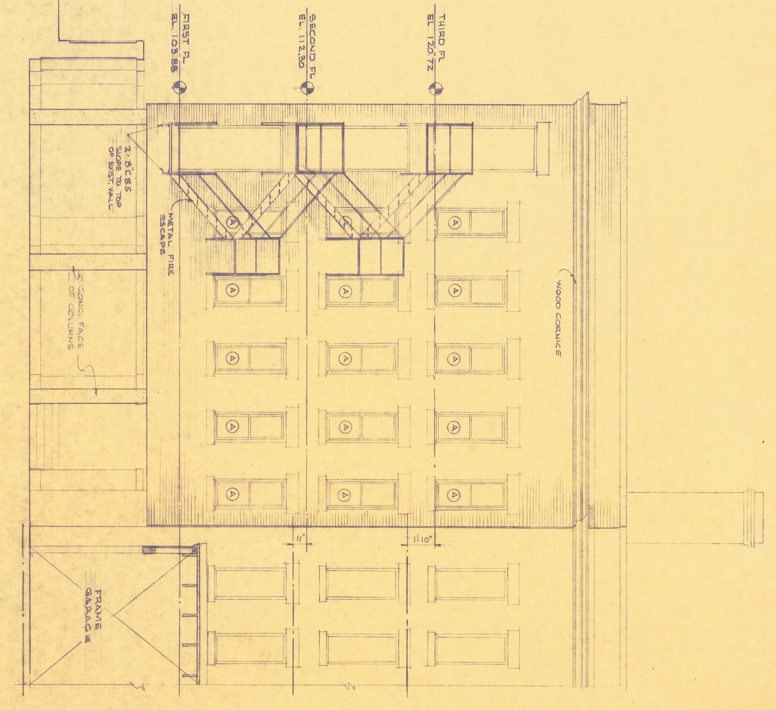
NORTHWEST ELEVATION 1/4" = 1'-0"
